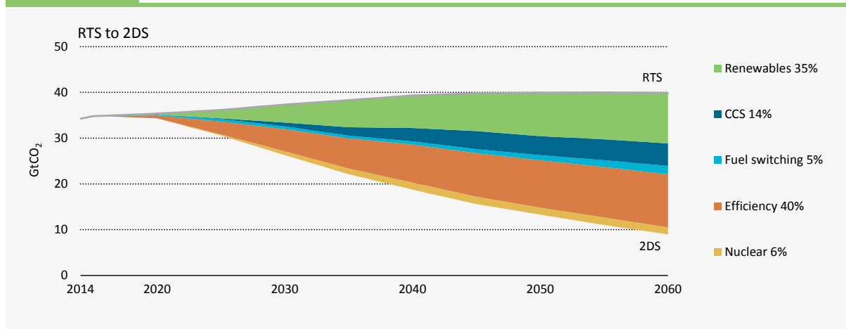
Figure 1.1. Sector contribution to emissions reduction
