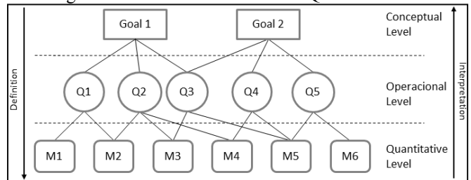
FIGURE 1. GQM STRUCTURE [7]
